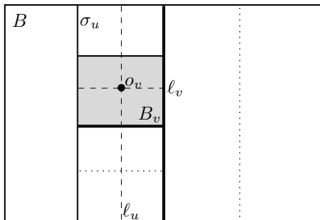
Figure 6: The rectangle B_v associated with a secondary node v , with its splitters and origin.
