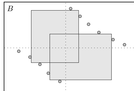
Figure 5: A set P of n points with \Theta(n^2) maximal P -empty rectangles.
