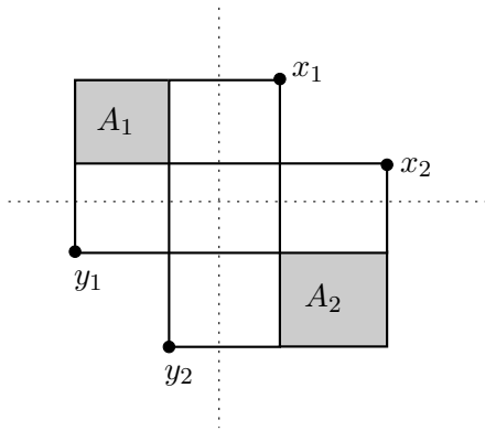
Figure 11: The inverse Monge property of maximal rectangles.
