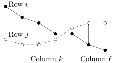
Figure 3: The pseudo-lines of two rows in an inverse Monge matrix.
