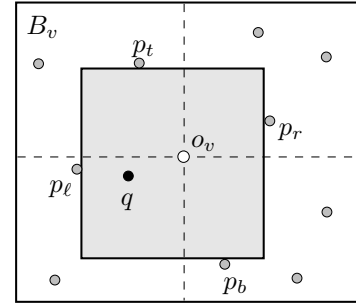
Figure 8: A bounded maximal P -empty rectangle with one defining point in each quadrant.
