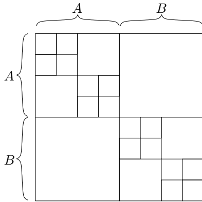
Figure 13: Illustration of the decomposition of M^{P,h,h} into Monge Submatrices.
