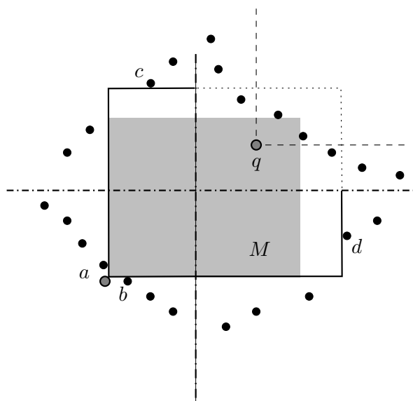
Figure 9: The structure of maximal empty rectangles with two defining points in each of the first and third quadrants.
