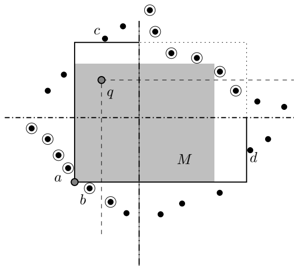
Figure 12: Querying with a point in the second quadrant. The highlighted points form the prefixes E_q and F_q , plus one extra point in each chain.
