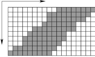
Figure 10: The structure of the defined portion of A .
